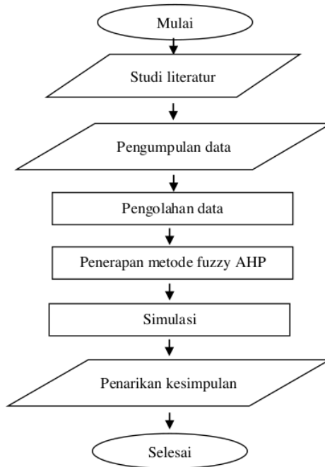
Gambar 1. Flowchart Sistem
