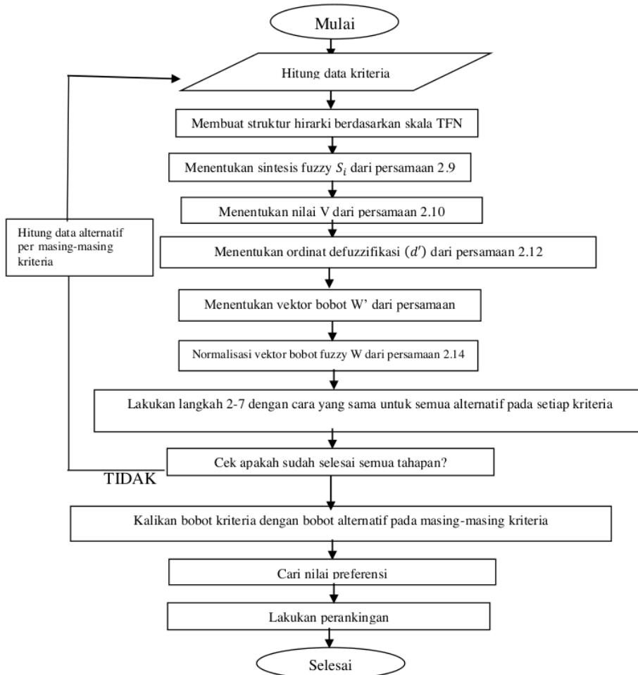
Gambar 2. Flowchart AHP
