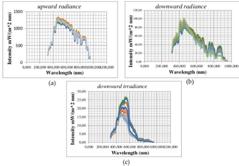
Figure 3. Graph of water upward radiance (a), downward atmosphere radiance (b), and downward irradiance (c).
