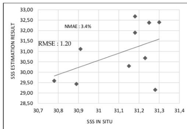
Figure 4. The correlation of the estimated and the in-situ SSS using other algorithms.
