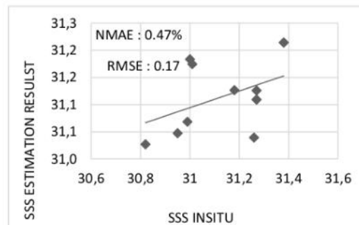
Figure 6. In-situ and estimated SSS correlation: new algorithm.
