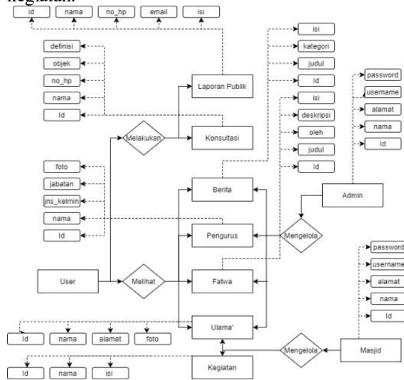
Gambar 3. Entity Relationship Diagram (ERD) MUI Kabupaten Pamekasan
