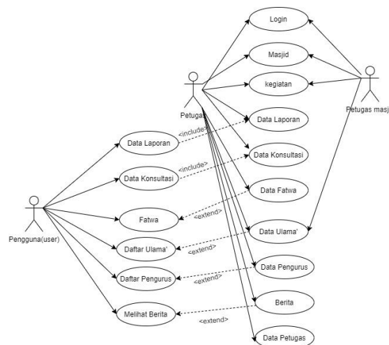
Gambar 2. Use Case Diagram Web MUI
