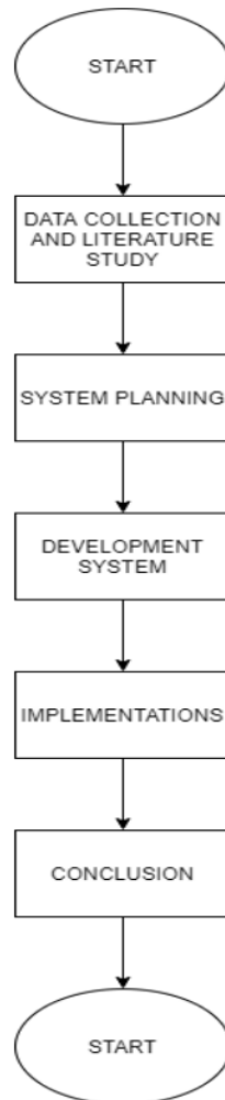
Figure 2.1. Research Stage
