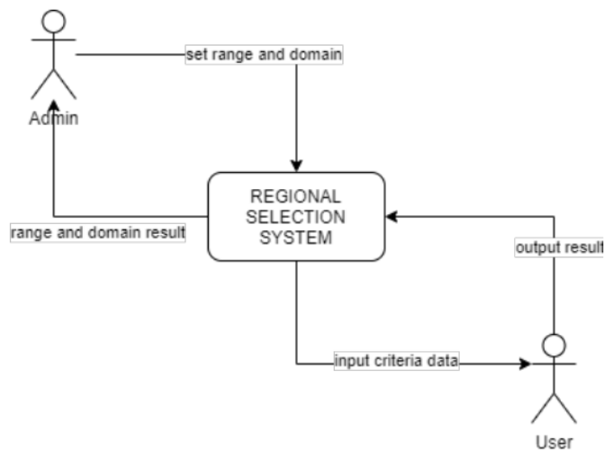
Figure 3.1. Context Diagram
