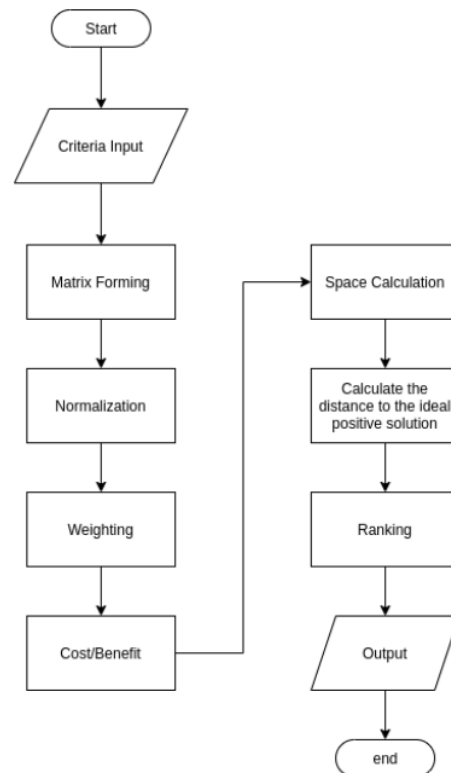
Figure 5. Flowchart
