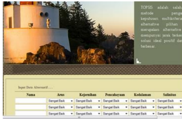
Figure 7. Alternative Page
