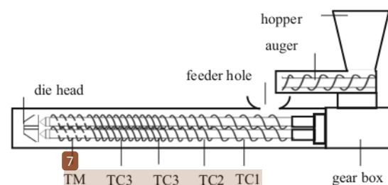
7. Scheme modular barrel and profile of twin screw extruder (Berto Industry BEX-DS-2256). TC = groove transfer direct pitch element (TC1 = 300 mm, TC2 = 220 mm, TC3 = 140 mm, TC4 = 120 mm). TM = groove mixing pitch element (80 mm), total long screw = 800 mm)
