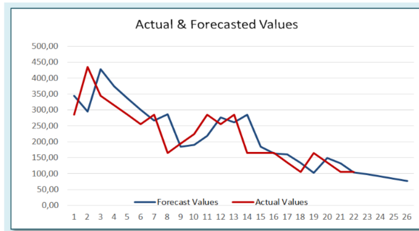
Figure 5. Fuzzy Double Exponential Smoothing Forecasting Results
