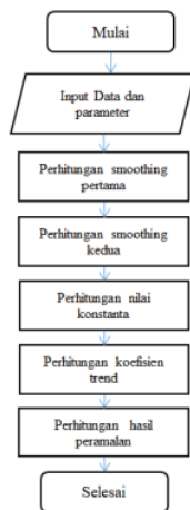
Gambar 2. Diagram alir Double Exponential Smoothing
