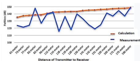
Fig 4. NLOS Transmission Path Loss Value Against Distance at Frequency 28 GHz
