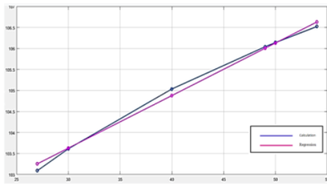
Fig 9. Graph of Calculation and Prediction of path loss to distance on frequency 73 GHz and LOS condition
