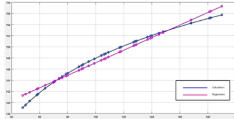
Fig 10. Graph of Calculation and Prediction of path loss to distance on frequency 73 GHz and NLOS conditions
