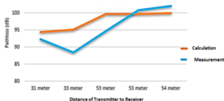
Fig 3. LOS Transmission Path loss Value Against Distance at Frequency 28 GHz
