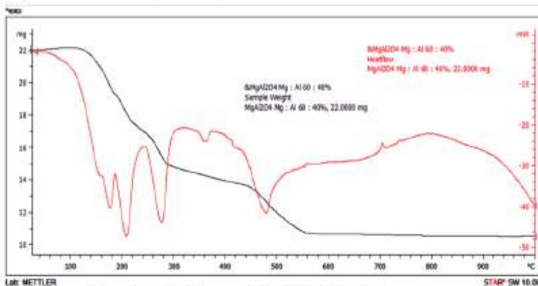
Figure 1. DSC-TGA curve of MA46 (40%:60%) dried sample. The heat rate was 10 °C/min.
