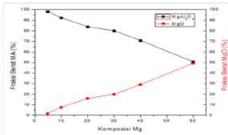
Figure 5. The relative weight fraction of MA phases samples for various Mg-to-Al compositions at 650 °C.
