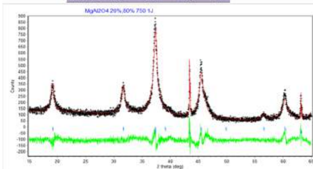
Figure 4. Typical Rietveld refinement plot using Rietica from the MA2080 sample. The observed pattern is described by (++) symbol while the calculated pattern by a red straight line. The bottom green curve is a plot of the difference between the measured and calculated patterns. Small vertical straight lines represent diffraction peak positions.
