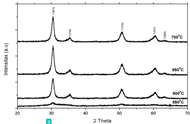
Figure 4. XRD results of synthesis of ZrO 2 from natural zircon sand of Kereng Pangli for precipitation at pH 10.
