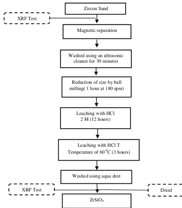
Figure 1. Flow Chart of Zircon Sand ( ZrSiO_4 ) Purification
