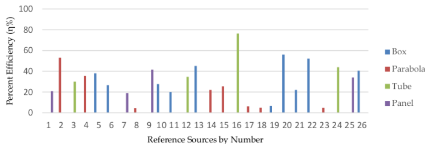
Figure 8. Review Of Percent Efficiency ( \eta\% ) Based on Solar Cooker Type
