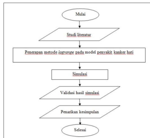
Gambar 1: Flowchart Penelitian
