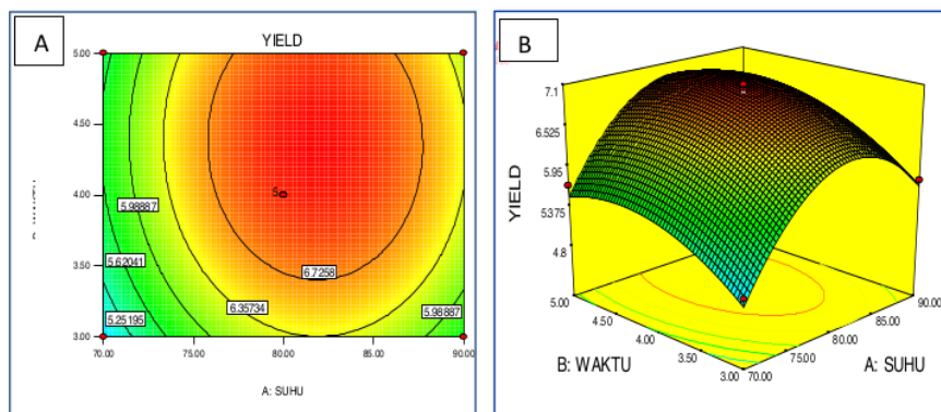
Figure 1. (A) Contour Plot (B) Graph of the effect of temperature and extraction time on the fucoidan yield of Sargassum sp.
